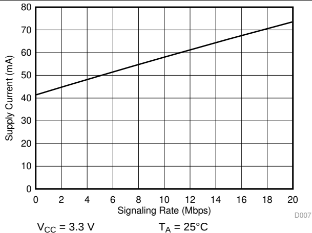
Figure 12. SN65HVD73, SN65HVD74 Supply Current vs Signal Rate
