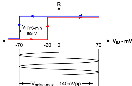
Figure 18. Noise Immunity
