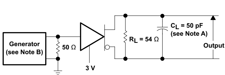
TEST CIRCUIT
