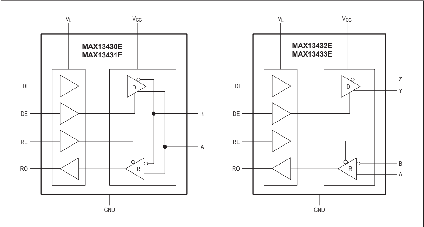
Figure 9. Functional Diagrams
